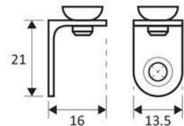
AK-06 Ambalan Karet Material : Besi Plat Finish : Galvanized
