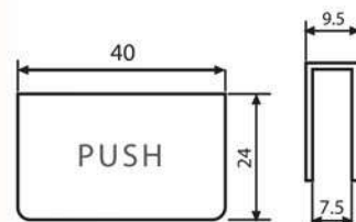
PS-17 Push Single Material : Plat Besi Finish : Chrome
