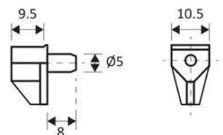
AB-5 Ambalan Bening Material : Besi & Plastik Finish : Galvanized
