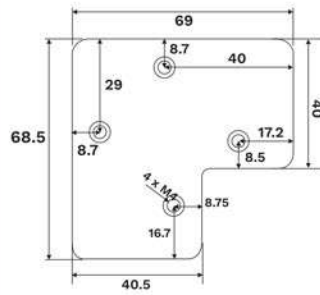
AH-45 Siku Frame Aluminium Material : Plat Besi
