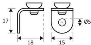
AKP-15-SS Ambalan Kaca Plat Material : Stainless Steel Finish : Nickel
