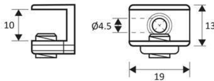
AKP-15-SS Ambalan Kaca Plat Material : Stainless Steel Finish : Nickel
