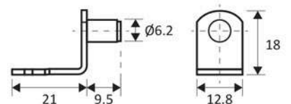
AK-06 Ambalan Karet Material : Besi Plat Finish : Galvanized
