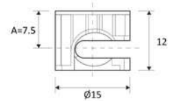
MF-15-G Casing Minifix Material : Zinc Alloy
