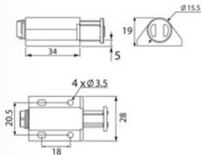
MS-31 Magnet Single
