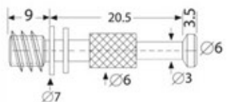
DU-6249 Skrup Minifix Material : Besi
